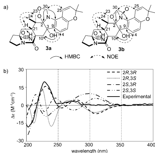
Figure 4. a) Key HMBC and NOE correlations for two possible structures of 3 . b) Experimental ECD spectrum of 3 along with calculated ECD spectra of 2 R ,3 R -, 2 R ,3 S -, 2 S ,3 R -, and 2 S ,3 S - 3a after optimization at the B3LYP/6-31G* level of theory.
