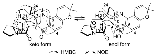
Figure 3. Key HMBC and NOE correlations for 2 .
